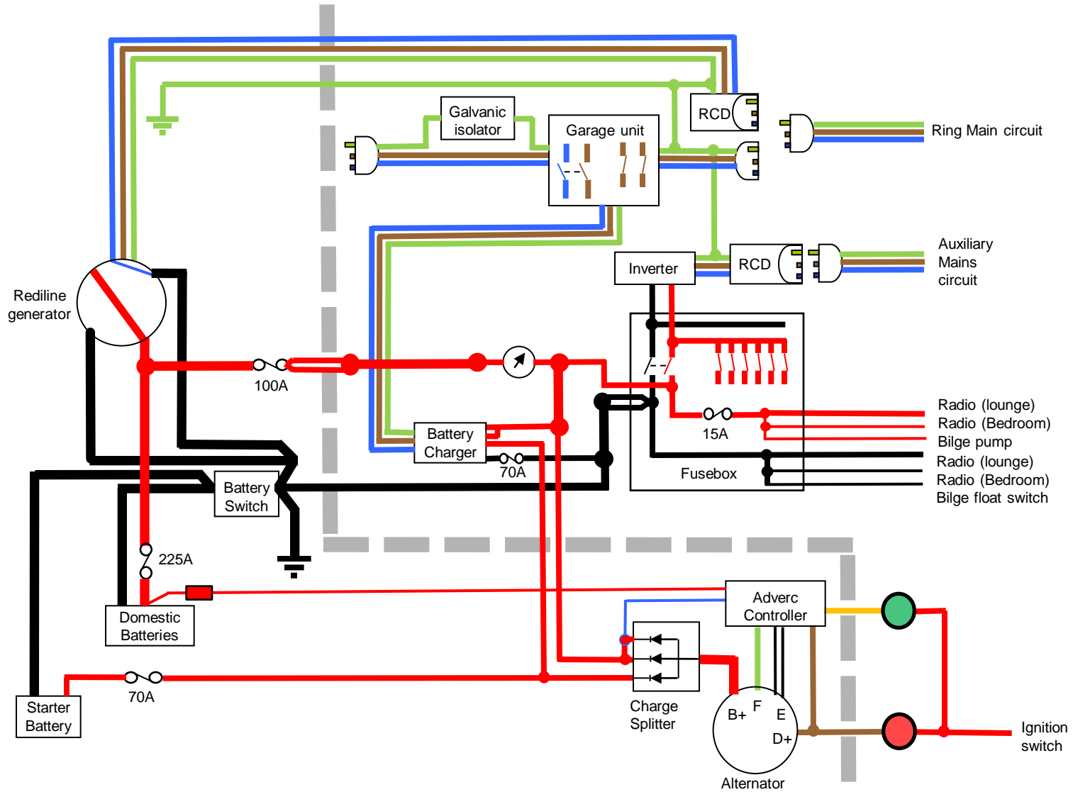
Keeping Up: AC and DC power wiring
